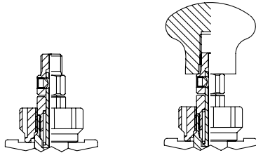
PULL STYLE CABLE OPERATED HAND OPERATED
