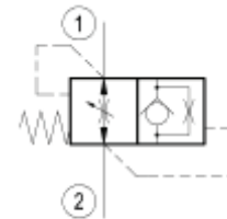
Hose burst valve with orifice
